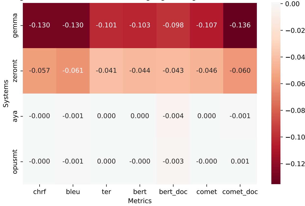
Average Score Differences Across Languages (Original – Bad Reference)
